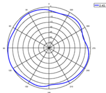
2.4G (Horizontal)
